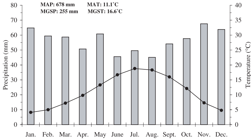
Figure 1. Climatic diagram for Le Mans (47° 56' 49,3'' N, 00° 11' 40,5'' W, 51 m). Mean monthly temperatures (°C ; line) and precipitations (mm ; bars) were calculated for the period 1961–1990. MAP, MGSP, MAT and MGST = Mean Annual or Growing Season (May to September) Precipitation and Temperature.
